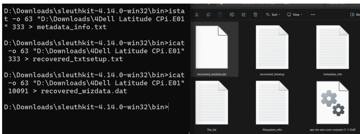
Figure 6: Successful extraction and recovery of wizdata.dat using the icat command
